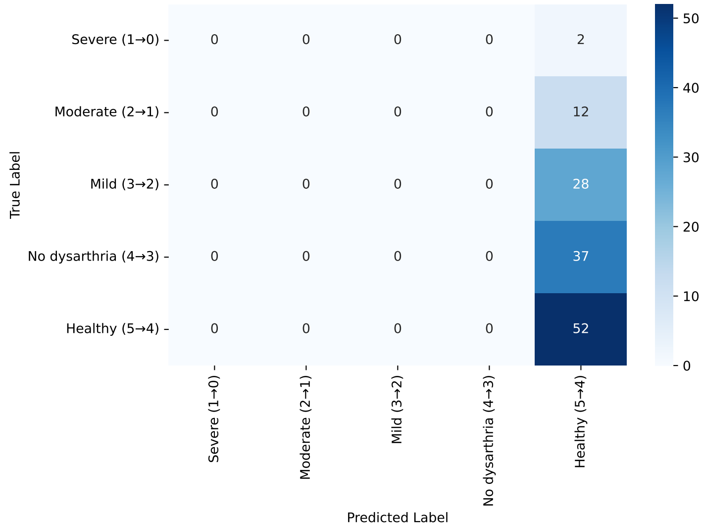
Confusion Matrix - Whisper-tiny
